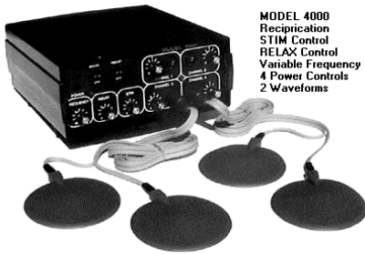
MODEL 4000 Reciprocation STIM Control RELAX Control Variable Frequency 4 Power Controls 2 Waveforms
